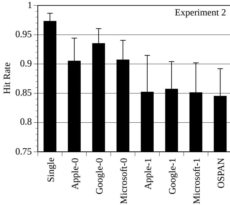
Figure 10. Mean DRT Hit Rate (an accuracy measure computed by determining the number of valid responses divided by the total number of responses) for the single-task, OSPAN, and off-task (e.g., Google-0) and on-task (e.g., Google-1) performance for the Apple, Google, and Microsoft secondary tasks in Experiment 2. Error bars reflect 95% confidence intervals around the point estimate.
