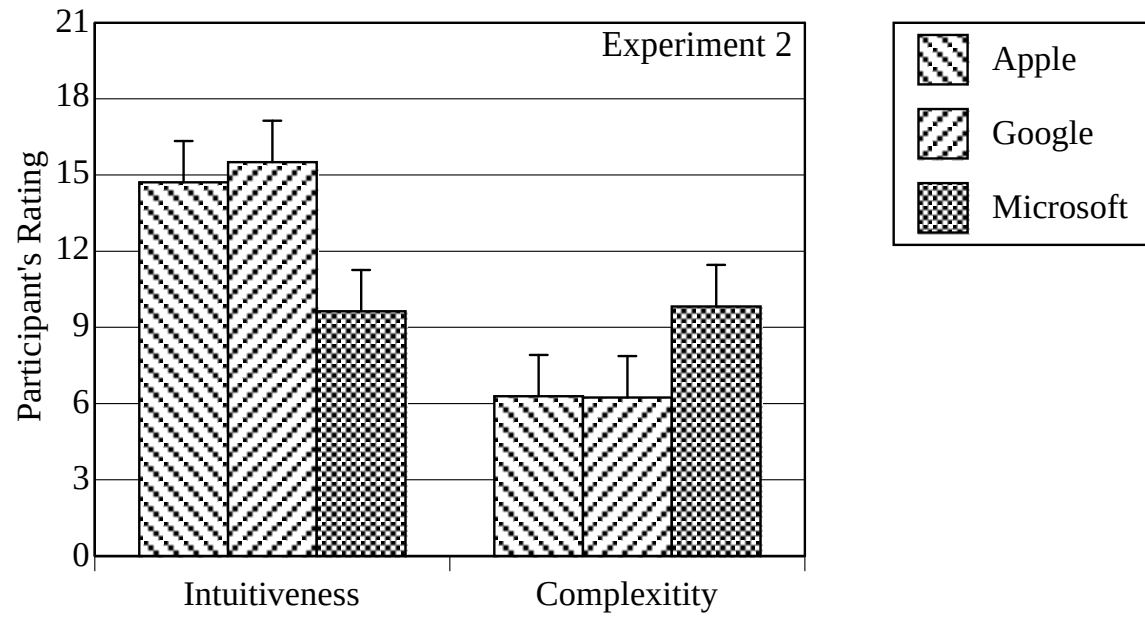
Figure 12. Mean ratings of intuitiveness and complexity for the Apple, Google, and Microsoft systems in Experiment 2. Error bars reflect 95% confidence intervals around the point estimate.
