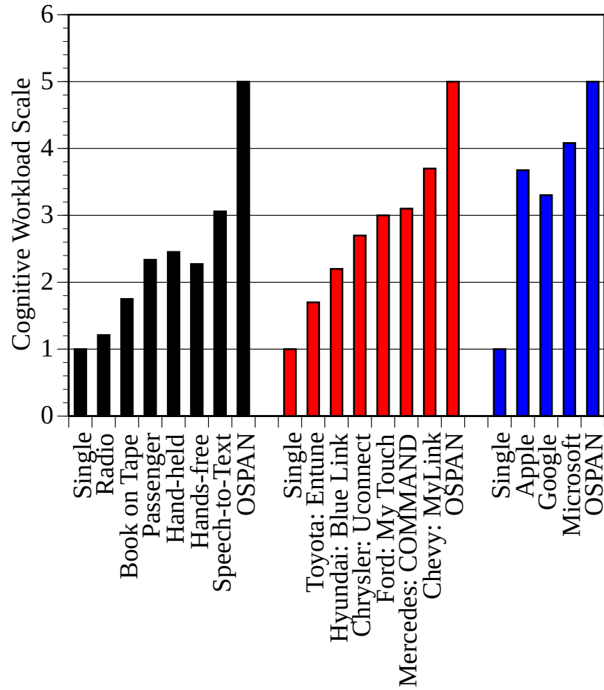
Figure 16. The workload scale for Strayer et al., (2013, the black bars), Cooper et al., (2014, the red bars), and the current research (blue bars).
