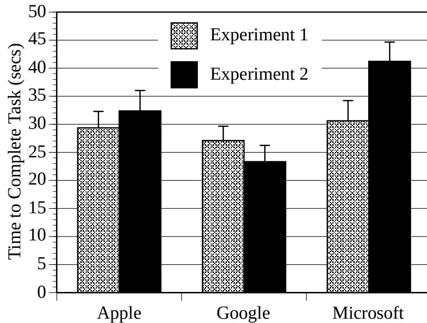
Figure 7. Average time to complete the secondary tasks for the Apple, Google, and Microsoft systems in Experiments 1 and 2. Error bars reflect 95% confidence intervals around the point estimate.
