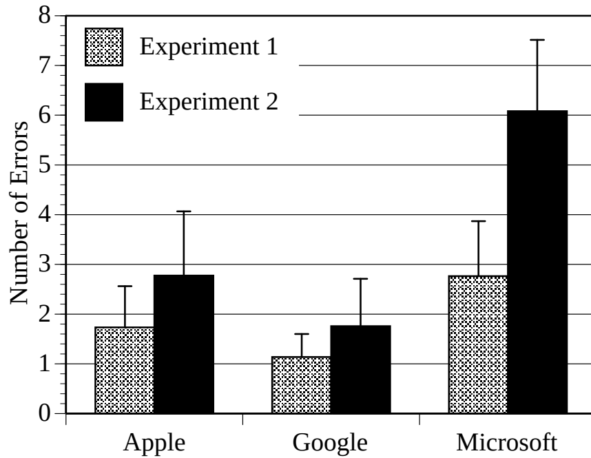
Figure 6. Average number of errors experienced by participants for the Apple, Google, and Microsoft systems in Experiments 1 and 2. Error bars reflect 95% confidence intervals around the point estimate.
