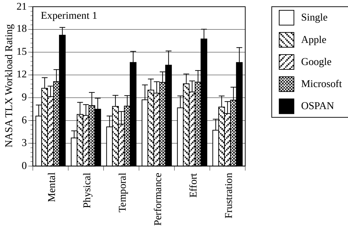
Figure 3. Mean NASA TLX ratings for the six sub-scales in the 5 conditions of Experiment 1. Error bars reflect 95% confidence intervals around the point estimate.
