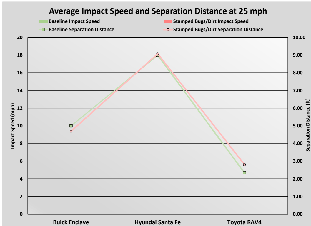
Figure 49: Average impact speed and final separation distance at 25 mph Image Source: AAA
