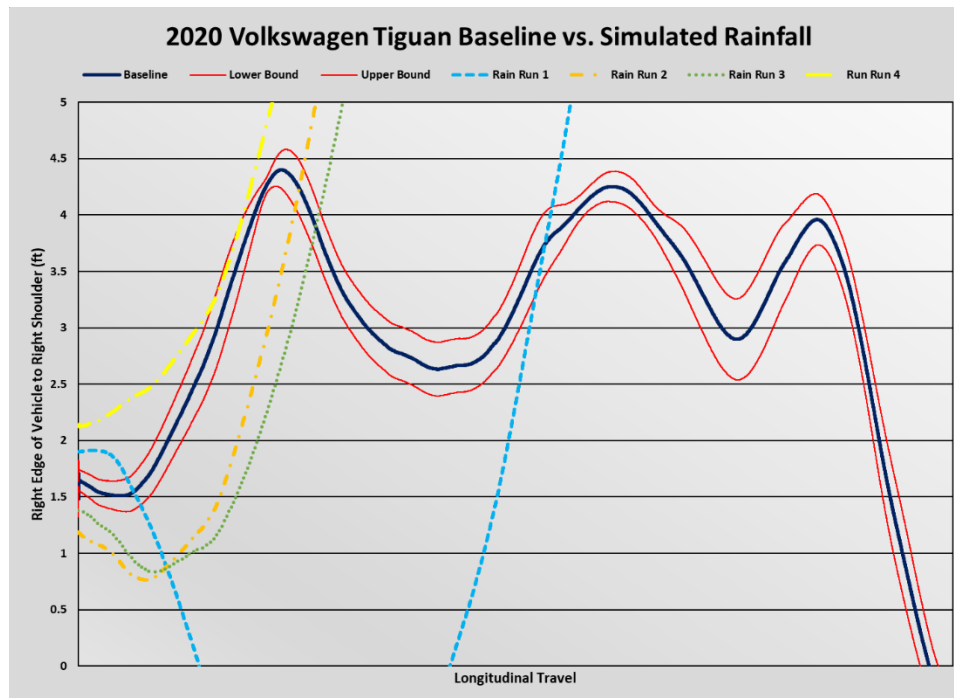
Figure 19: 2020 Volkswagen Tiguan average baseline lane placement and individual runs with simulated rainfall
