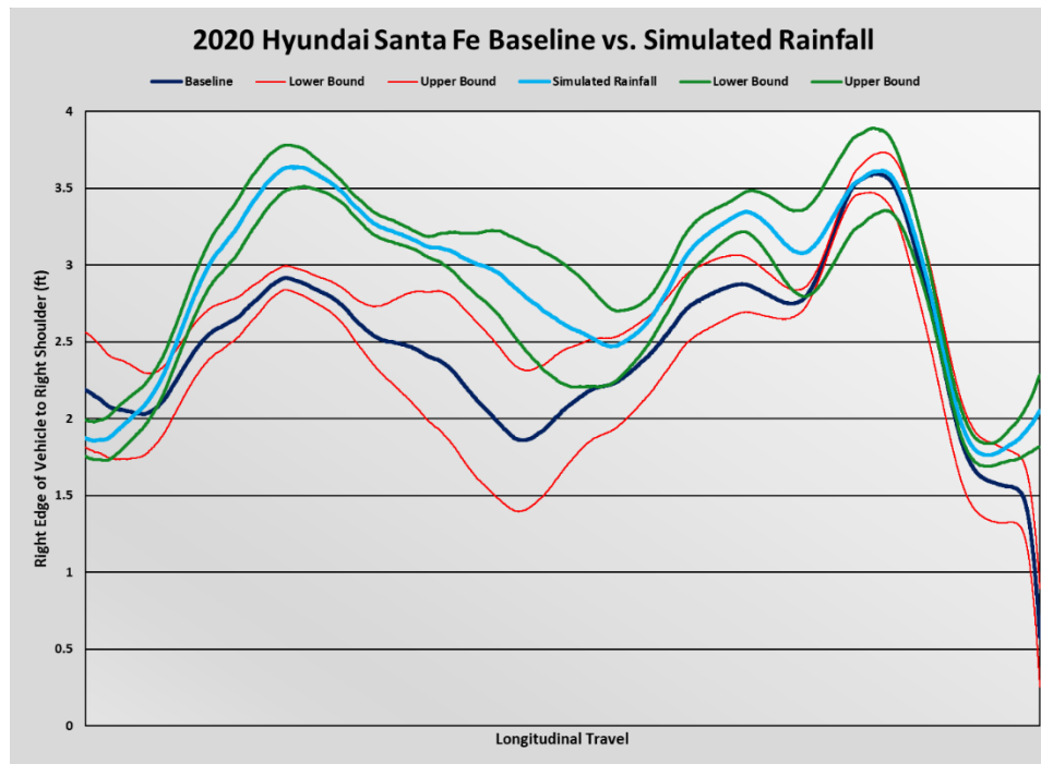
Figure 15: 2020 Hyundai Santa Fe averaged baseline and simulated rainfall lane placement Image Source: AAA
