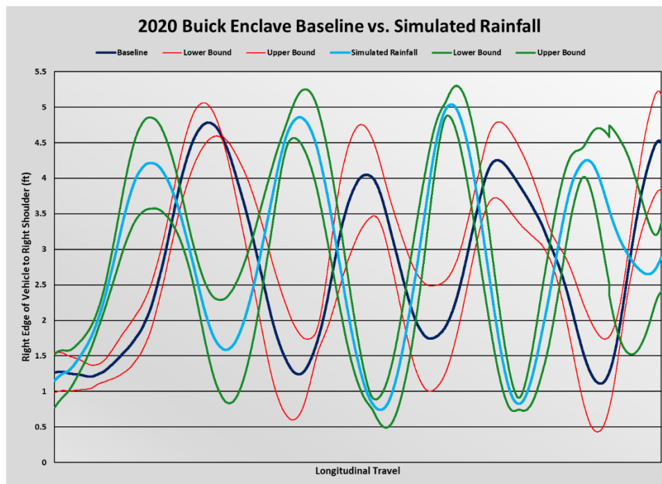
Figure 12: 2020 Buick Enclave averaged baseline and simulated rainfall lane placement
