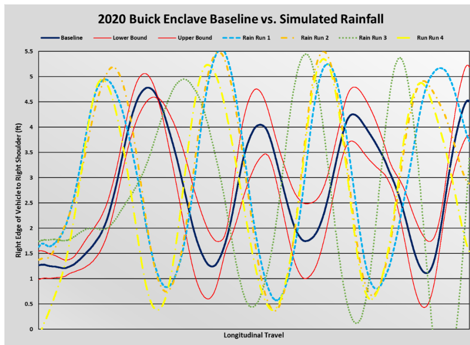
Figure 10: 2020 Buick Enclave averaged baseline lane placement and individual runs with simulated rainfall
