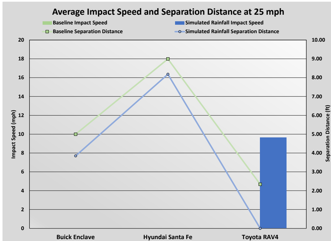
Figure 26: Average impact speed and final separation distance for each test vehicle at 25 mph Image Source: AAA
