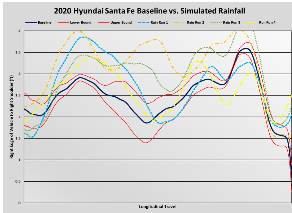
Figure 13: 2020 Hyundai Santa Fe average baseline lane placement and individual runs with simulated rainfall Image Source: AAA
