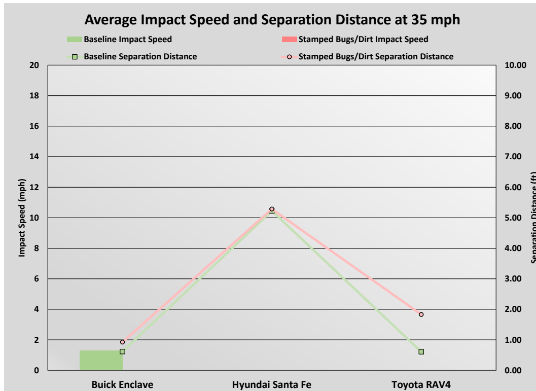
Figure 50: Average impact speed and final separation distance at 35 mph Image Source: AAA
