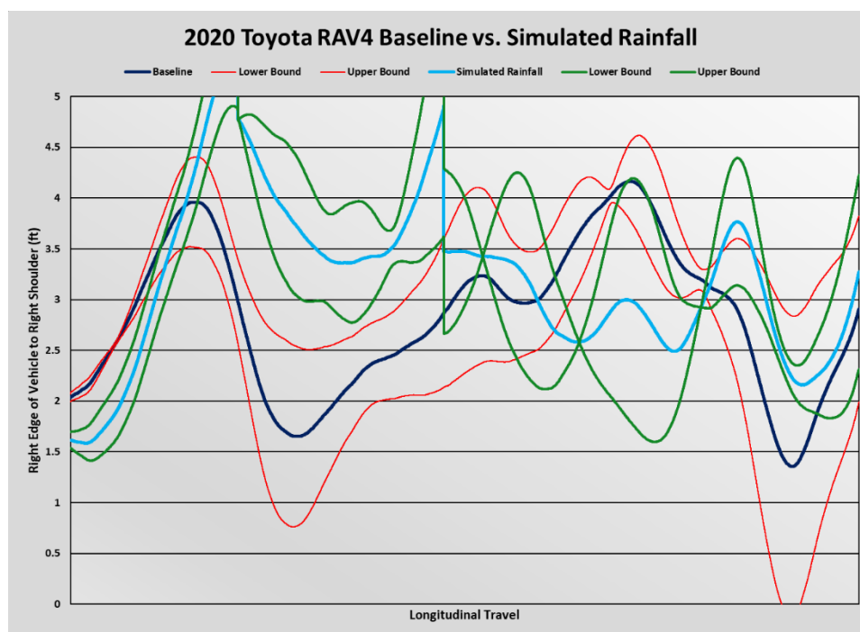
Figure 18: 2020 Toyota RAV4 averaged baseline and simulated rainfall lane placement Image Source: AAA
