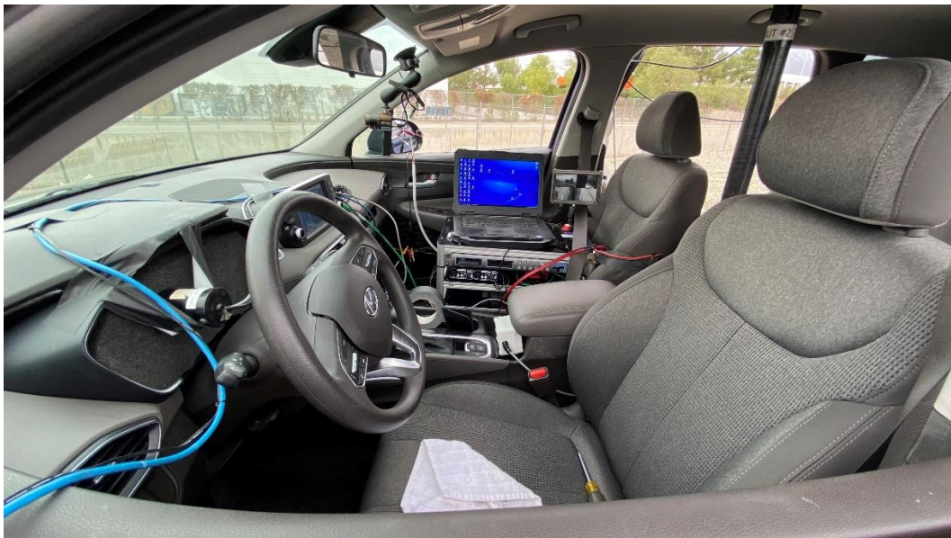
Figure 4: Data acquisition system and sensors installed in test vehicle Image Source: AAA
