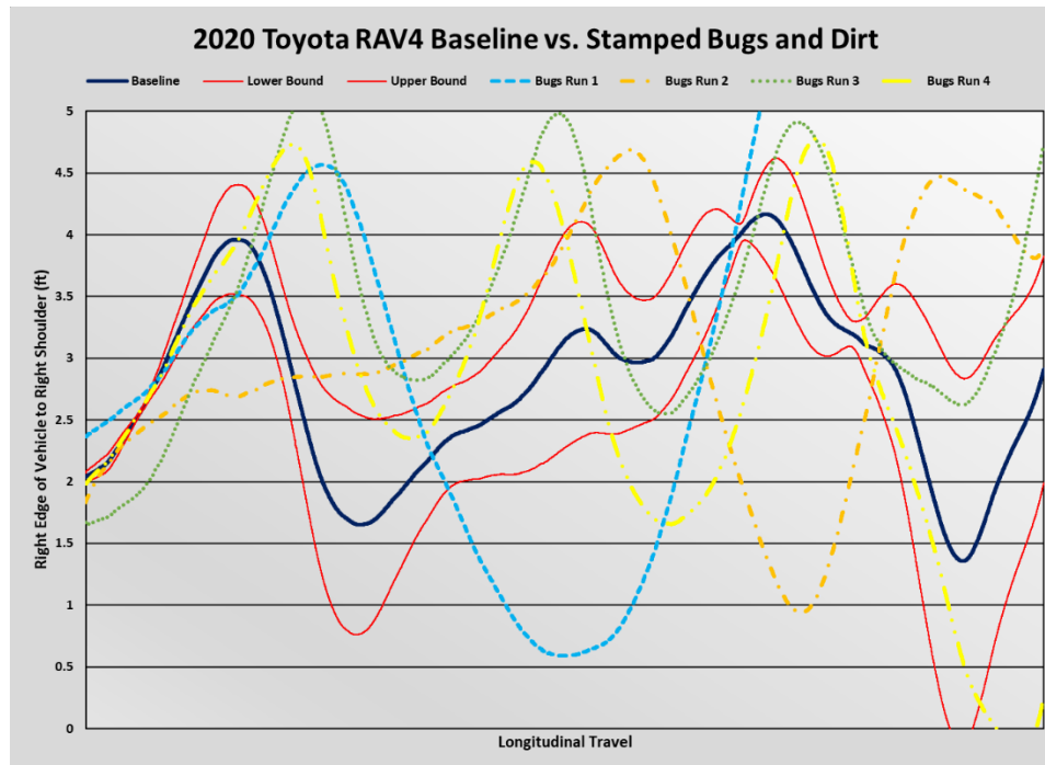
Figure 37: 2020 Toyota RAV4 average baseline lane placement and individual runs with occluded cameras Image Source: AAA
