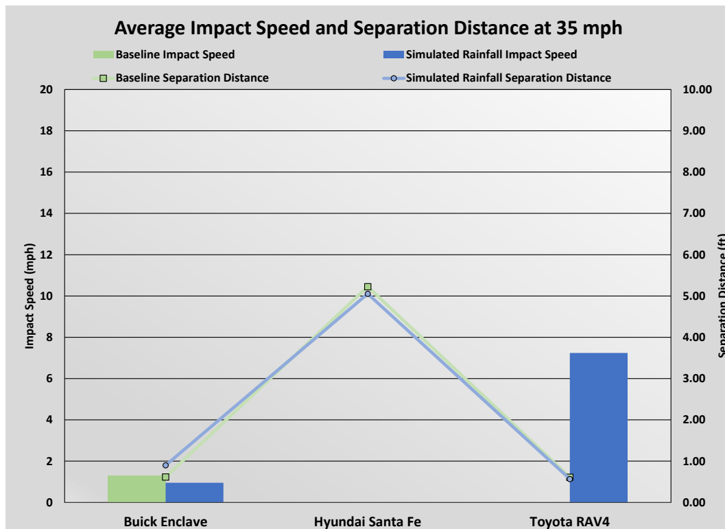
Figure 27: Average impact speed and final separation distance for each test vehicle at 35 mph
