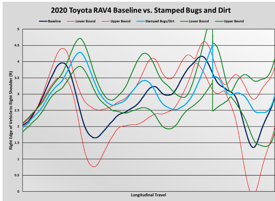
Figure 39: 2020 Toyota RAV4 averaged baseline and occluded cameras placement
