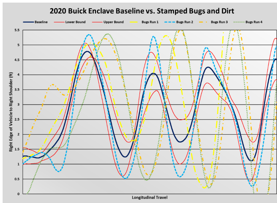
Figure 31: 2020 Buick Enclave average baseline lane placement and individual runs with occluded cameras Image Source: AAA
