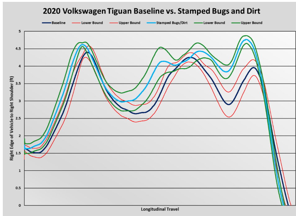
Figure 42: 2020 Volkswagen Tiguan averaged baseline and occluded cameras placement Image Source: AAA
