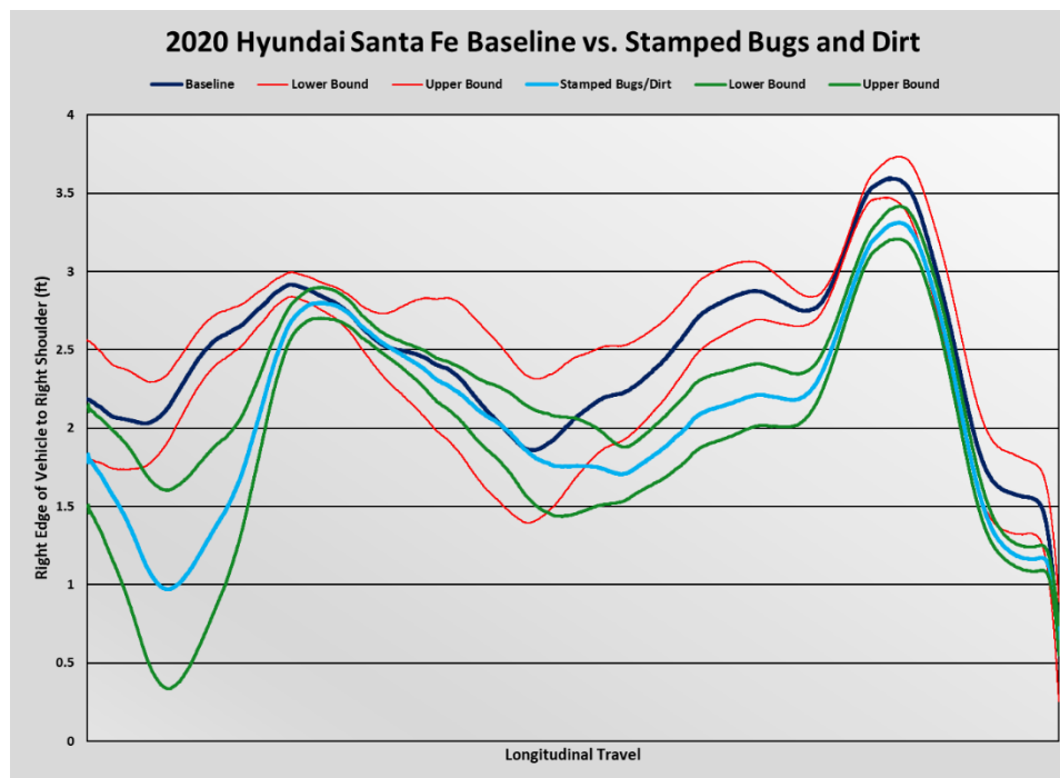
Figure 36: 2020 Hyundai Santa Fe averaged baseline and occluded camera placement
