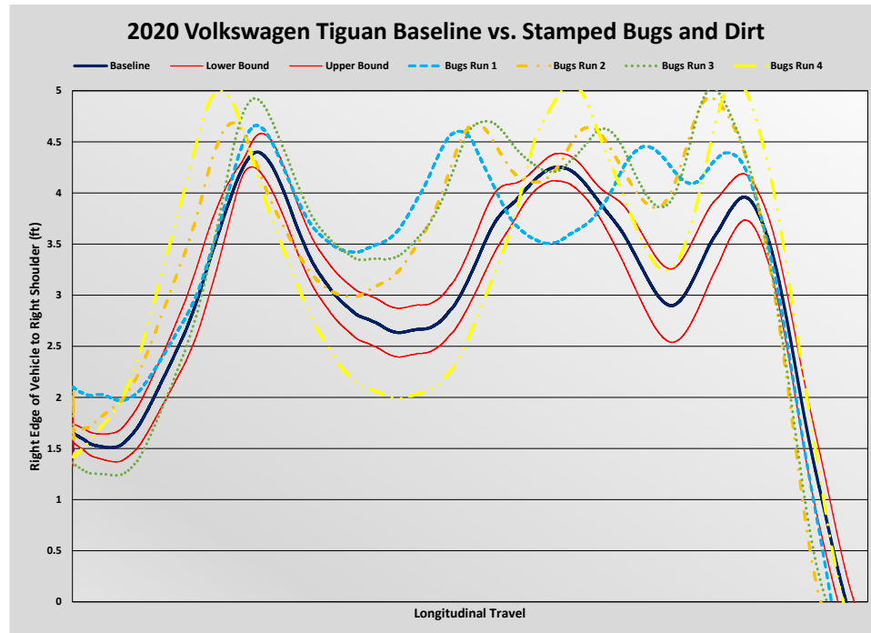
Figure 40: 2020 Volkswagen Tiguan average baseline lane placement and individual runs with occluded cameras Image Source: AAA
