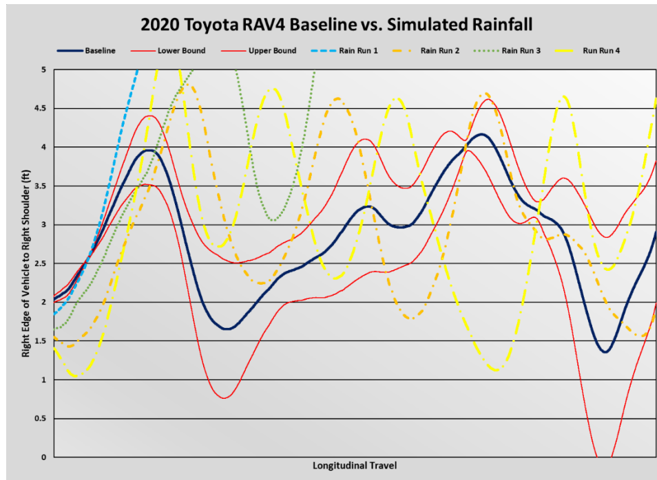
Figure 16: 2020 Toyota RAV4 average baseline lane placement and individual runs with simulated rainfall Image Source: AAA
