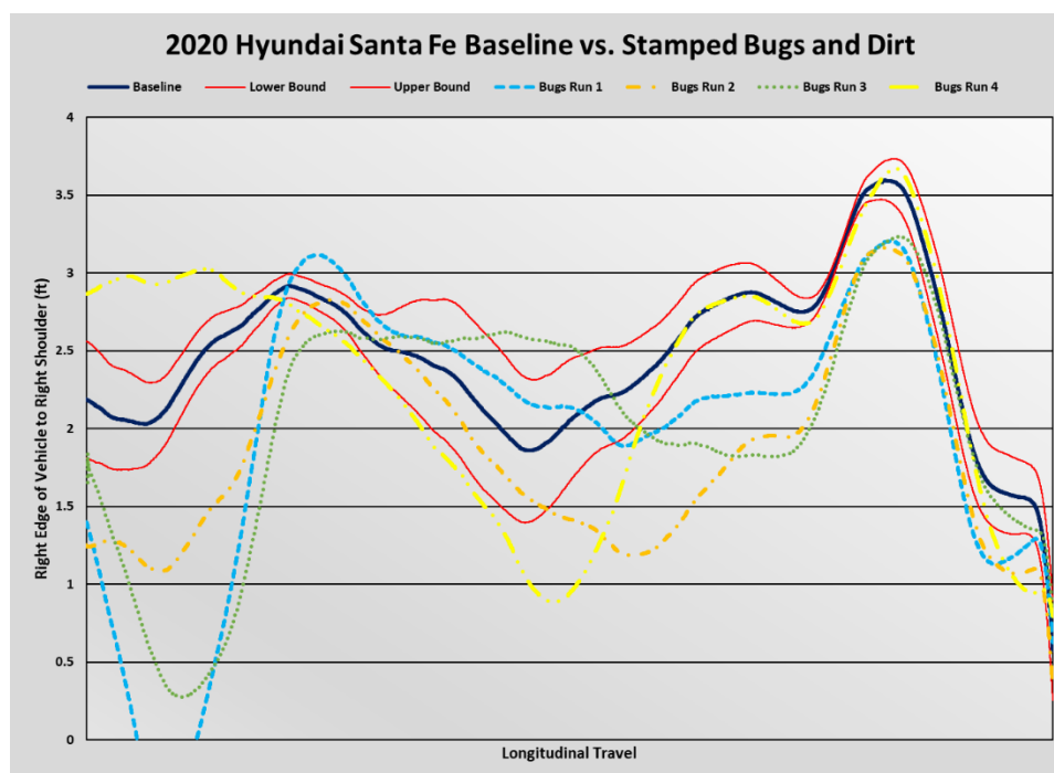
Figure 34: 2020 Hyundai Santa Fe average baseline lane placement and individual runs with occluded cameras Image Source: AAA
