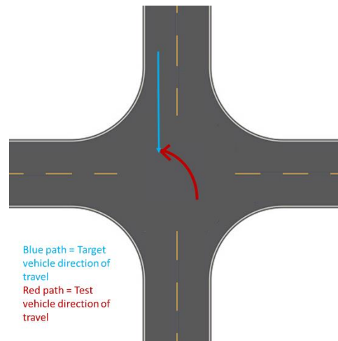
Figure 15: Turning collision scenario trajectory and impact point Image Source: AAA
