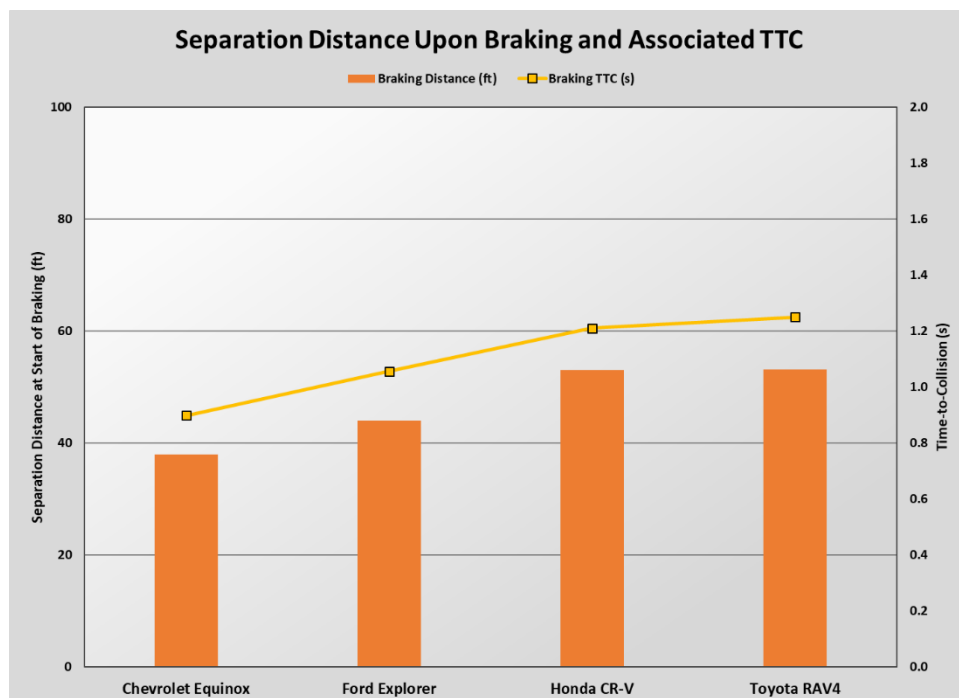
Figure 9: Average braking distance and associated TTC for each test vehicle Source: AAA
