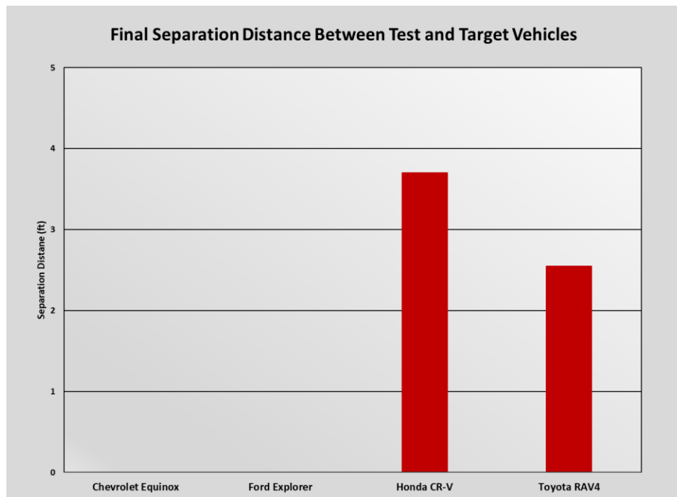
Figure 13: Average separation distance between test and target vehicles Source: AAA
