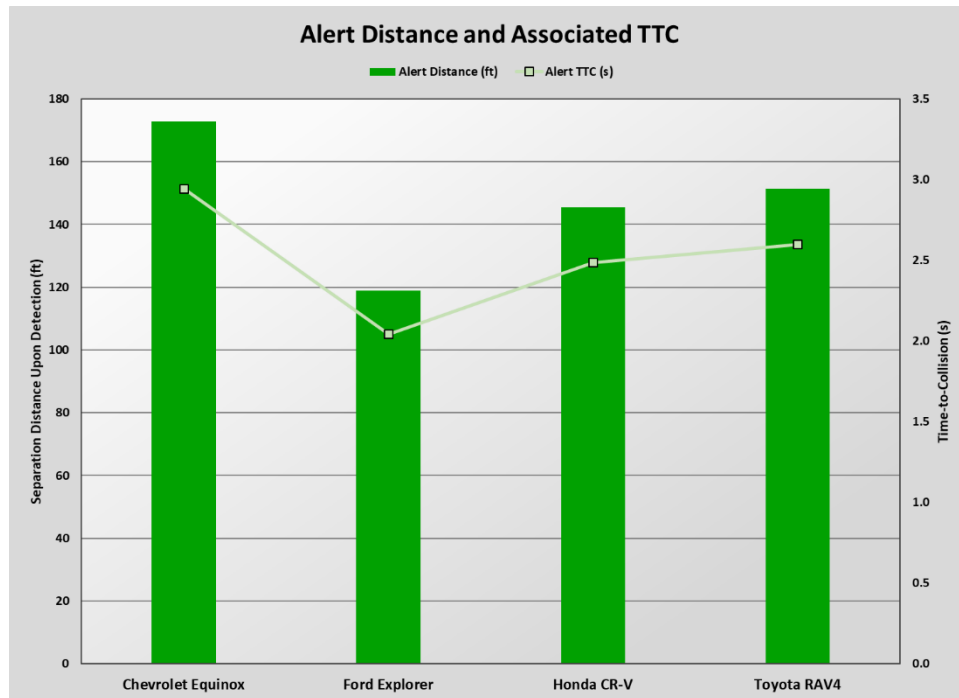
Figure 11: Average alert distance and associated TTC for each test vehicle Source: AAA
