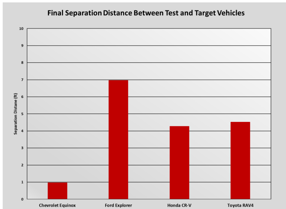
Figure 10: Average separation distance between test and target vehicles Source: AAA
