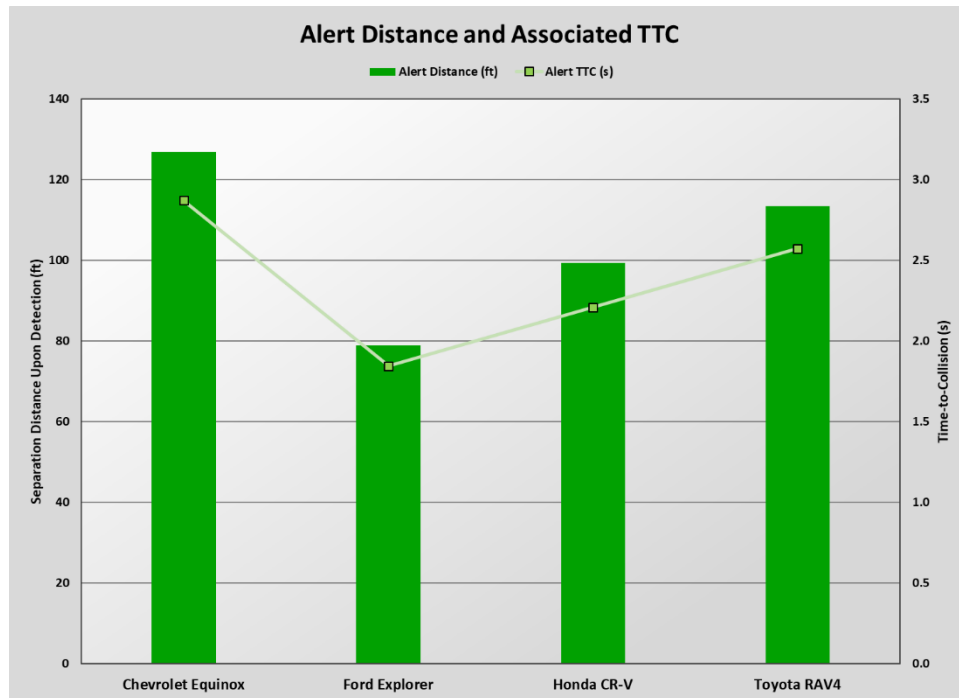
Figure 8: Average alert distance and associated TTC for each test vehicle Source: AAA
