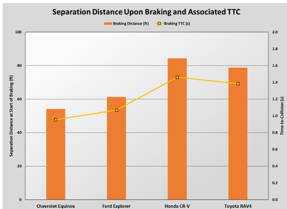
Figure 12: Associated braking distance and associated TTC for each test vehicle Source: AAA
